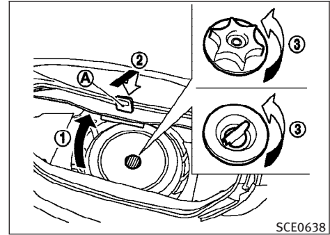
Spare tire
